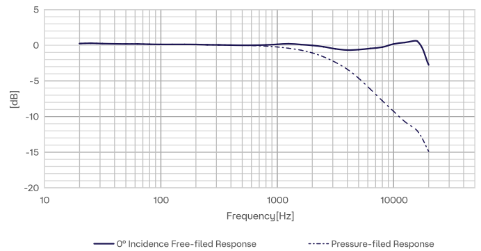
Fig.1 CRY3101-S01 Microphone Set Typical Frequency Response
