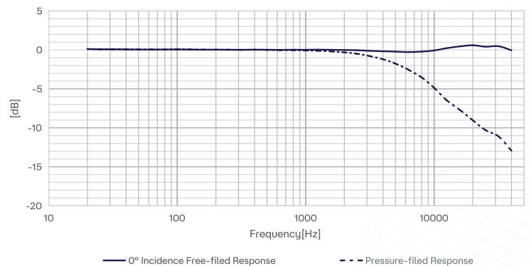
Fig.1 CRY3201-S01 Microphone Set Typical Frequency Response
