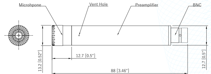
Fig.2 CRY3201-S01 Microphone Set Drawings
