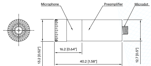
Fig.2 CRY3203-S02 Microphone Set Drawings
