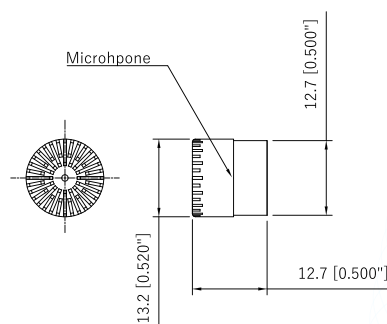
Fig.1 CRY3282 Microphone Drawings
