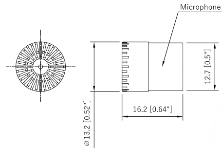
Fig.1 CRY3284 Microphone Drawings
