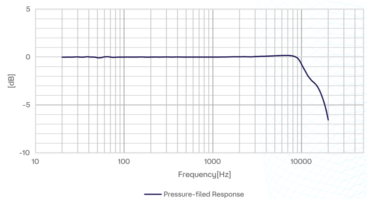
Fig.2 CRY3284 Microphone Typical Frequency Response
