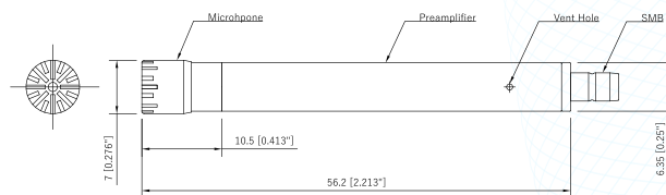
Fig.2 CRY3401-S01 Microphone Set Drawings
