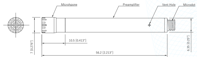
Fig.2 CRY3402-S02 Microphone Set Drawings
