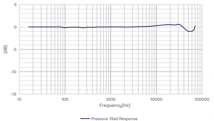
Fig.1 CRY3402-S02 Microphone Set Typical Frequency Response
