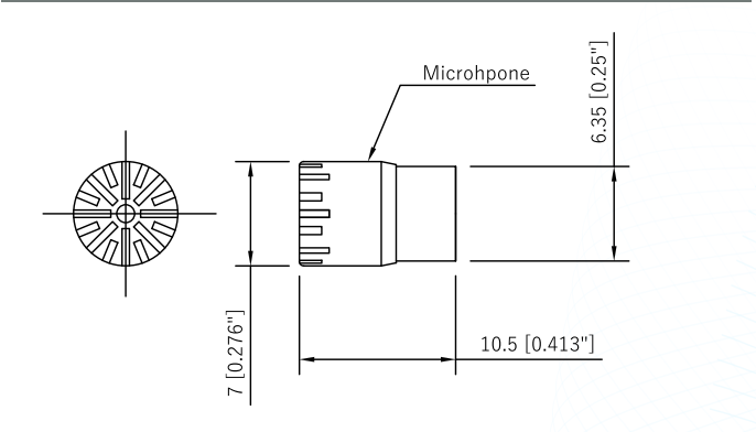
Fig.1 CRY3482 Microphone Set Drawings
