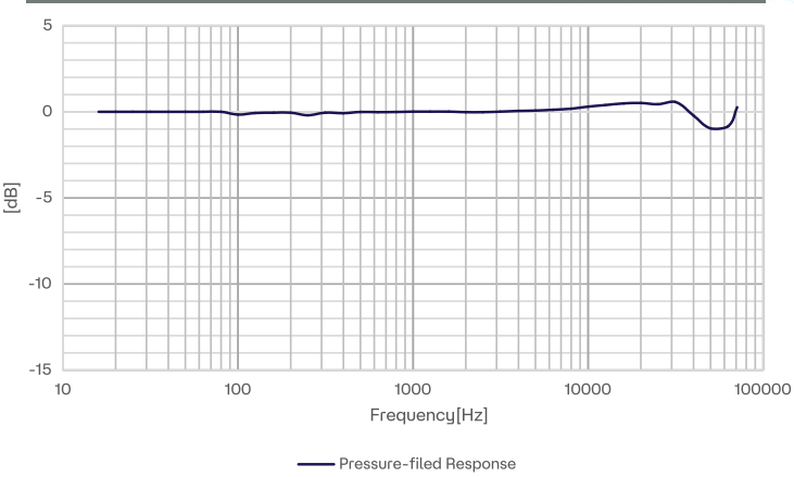
Fig.2 CRY3482 Microphone Typical Frequency Response
