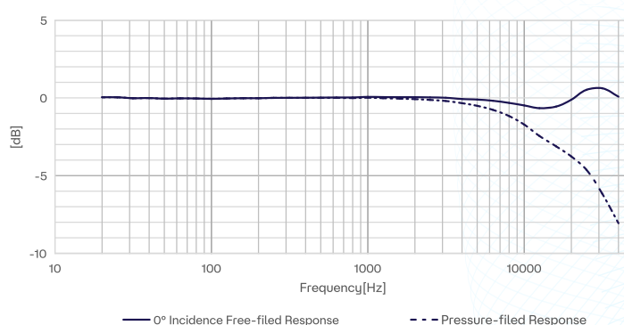
Fig.2 CRY3485 Microphone Typical Frequency Response
