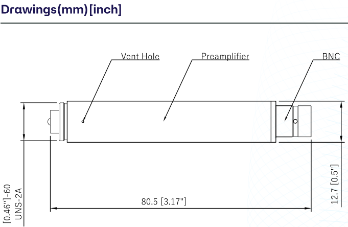
Fig.1 CRY3501 preamplifier Drawings
