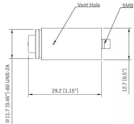
Fig.1 CRY3502 preamplifier Drawings
