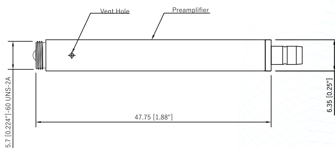
Fig.1 CRY3541 preamplifier Drawings
