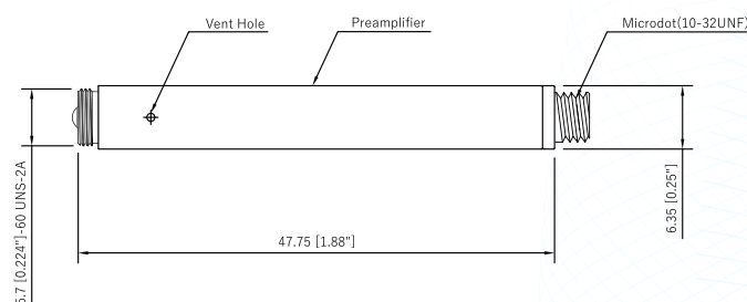
Fig.1 CRY3543 preamplifier Drawings
