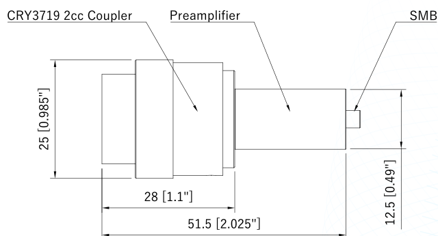
Fig.2 CRY3719-S01 Coupler Set Drawings
