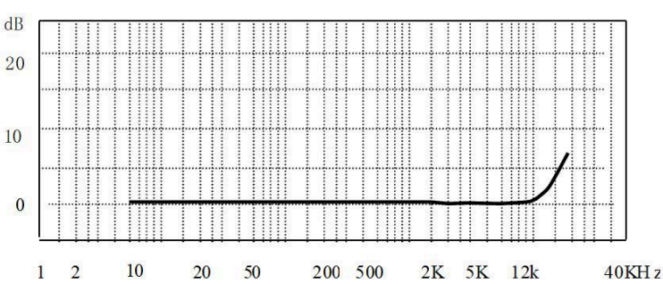
Fig.1 CRY431 Accelerometer Typical Frequency Response
