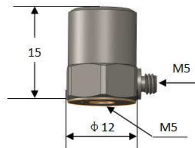
Fig.2 CRY432 Accelerometer Drawings
