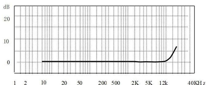
Fig.1 CRY432 Accelerometer Typical Frequency Response
