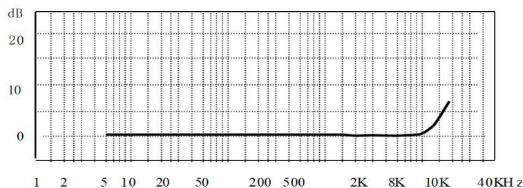
Fig.1 CRY434 Accelerometer Typical Frequency Response
